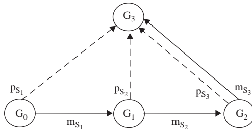
Fig. 10. G_3 farsightedly dominates G_0 .
