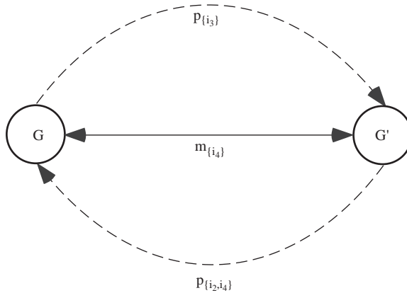
Fig. 9. The New Supernet G_2 .
